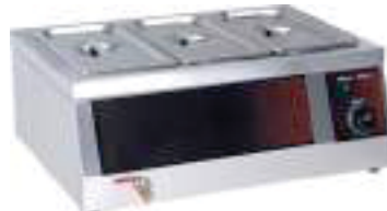
3 Pan (1/3 150mm) Size: 600x440x230mm Cap: 4Lx3 Power: 1.5Kw
